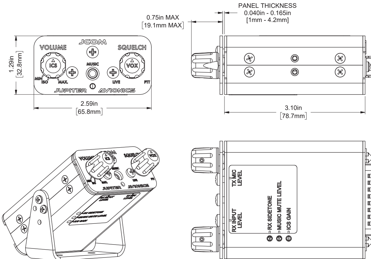
Optional Mounting Bracket INST-JA80BR
